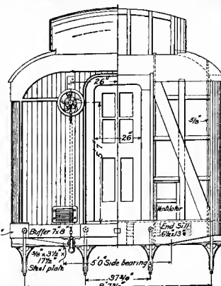
Fig. 585. End Elevation.
